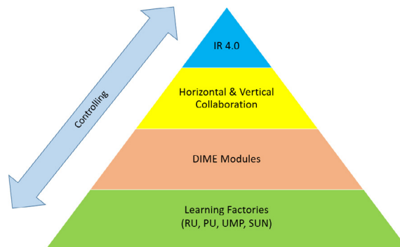
Fig. 1. Collaboration Framework.
