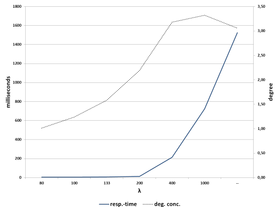
Figure 4. Response time and degree of concurrency for increasing \lambda for O|R|P|E .
